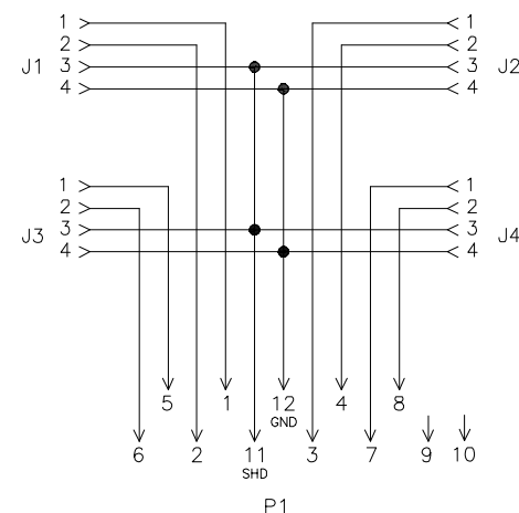
WIRING DIAGRAM
